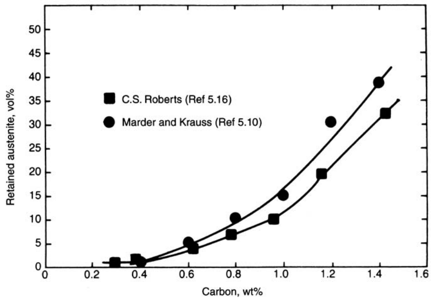
Retained austenite as a function of carbon content in Fe-C alloys. Source: Steels: Processing, Structure, and Performance, George Krauss, ASM International, p 64, 2005.
